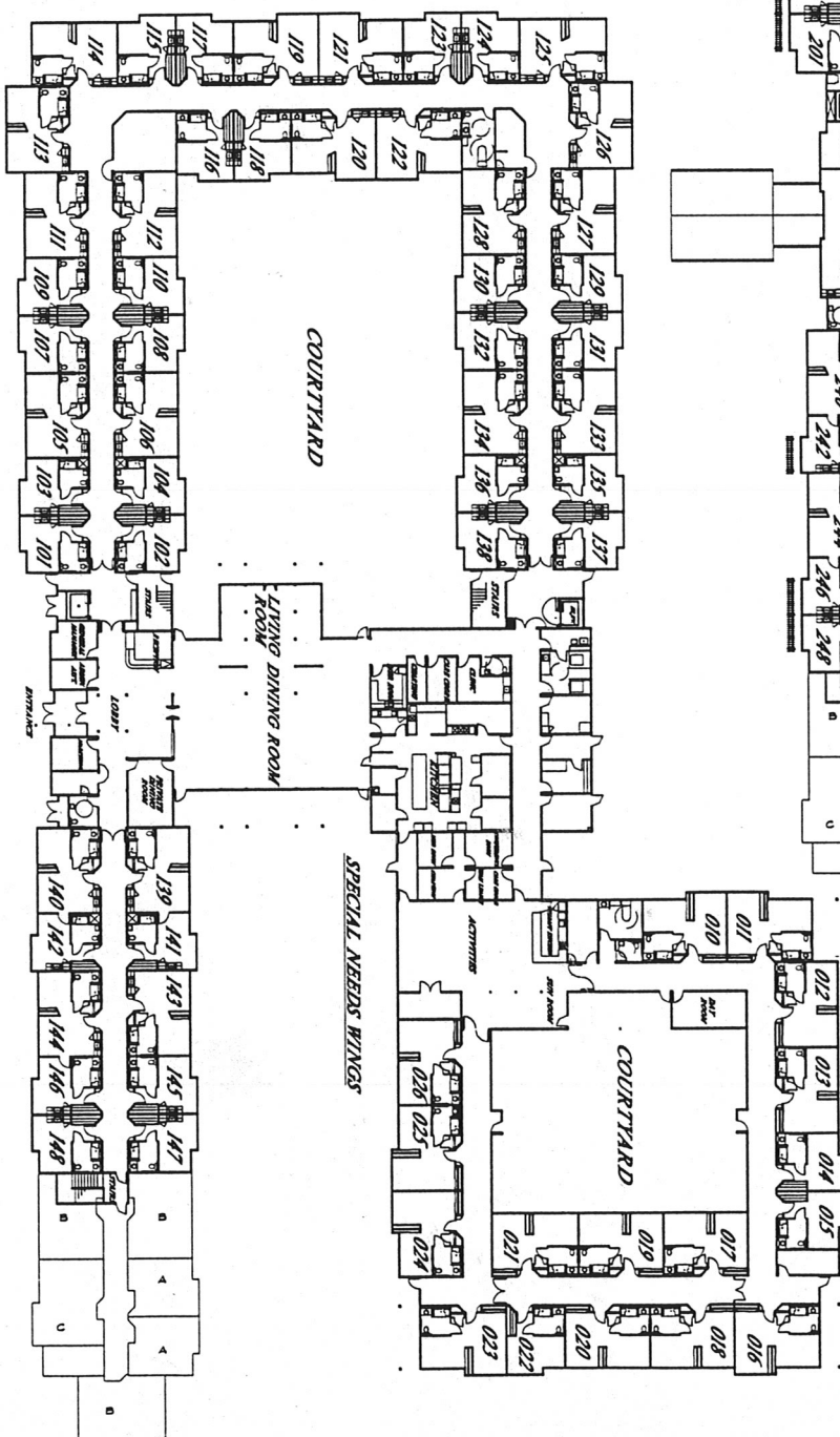
FIRST FLOOR
